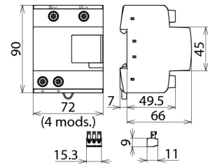
Dimension drawing DCB YPV SCI 1000 FM
