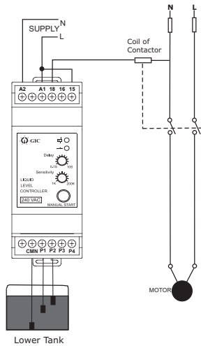
Draining Control (Single Tank Monitoring with 3 Sensors)
