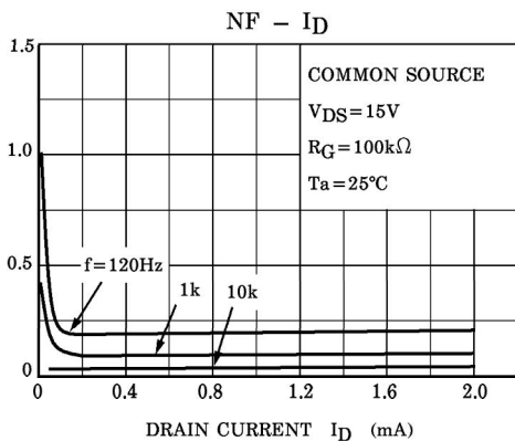
NOISE FIGURE NF (dB)
