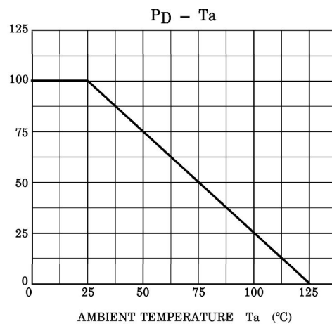
DRAIN POWER DISSIPATION P_D (mW)
