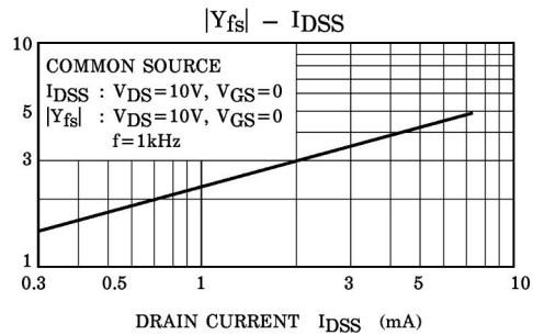
FORWARD TRANSFER ADMITTANCE |Y_{fs}| (mS)
